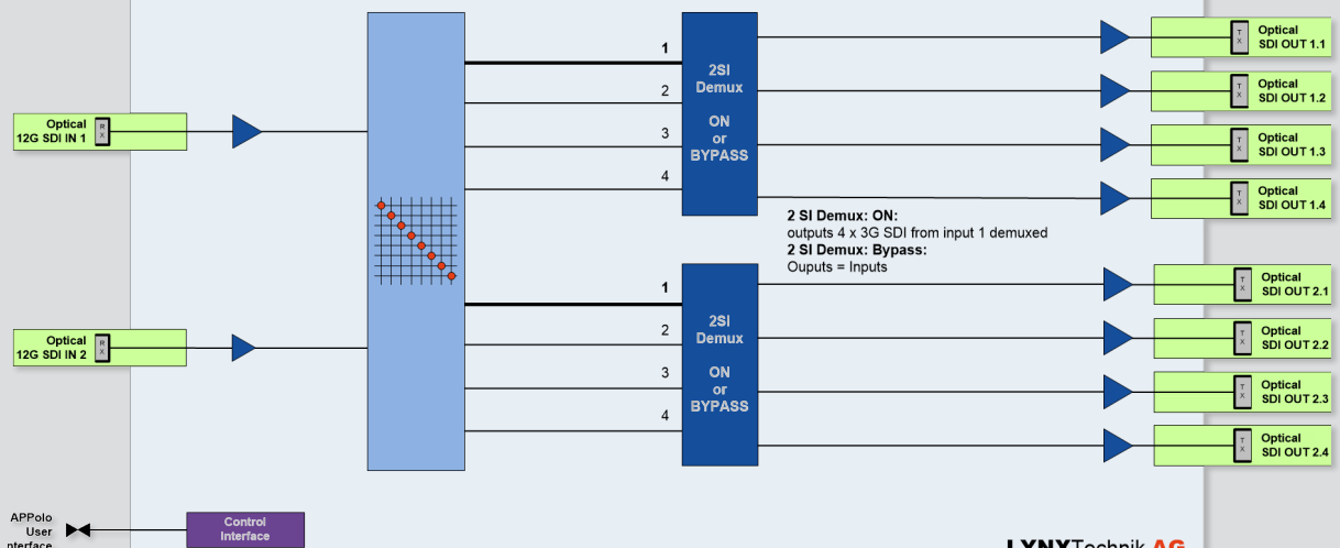
D VD 5480 TO – Dual 12G SDI Distribution Amplifier with 12G Single Link to Quad Link (2SI) conversion
