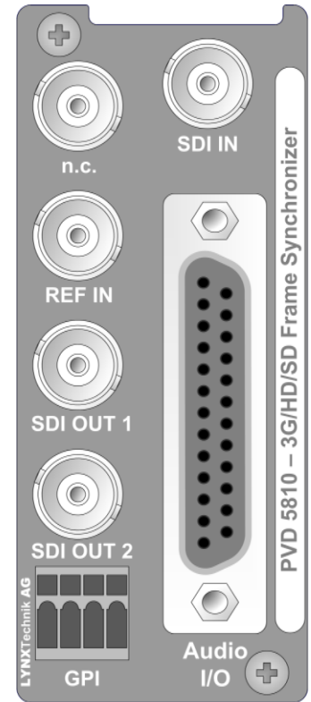
Figure 3: Rear Termination Panel P VD 5810-D
