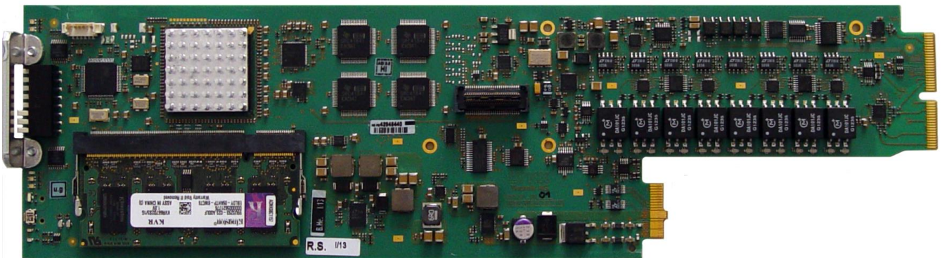
Figure 6: Board Layout
