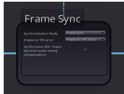
Figure 15: GUI Framesync
