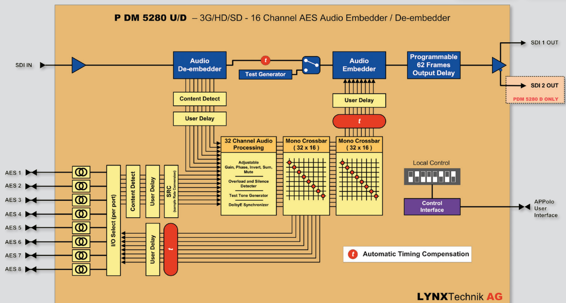
Two versions available: U = unbalanced AES on MiniDin connectors, D = balanced AES on Sub D connector
